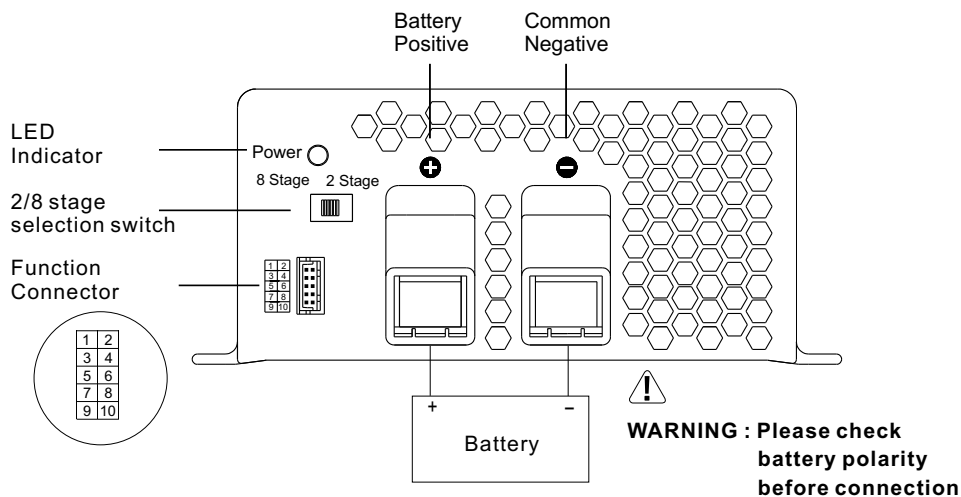
Figure 1.2 Back Panel
