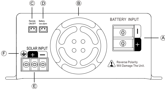
Figure 3.2 Rear Panel
