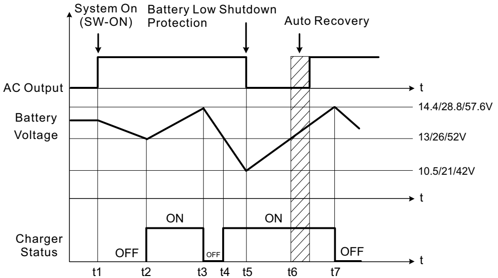
Figure 5.1 Operation Sequence
