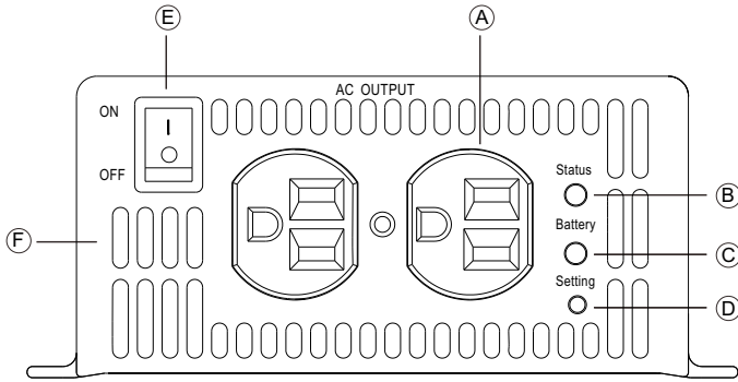
Figure 3.1 Front Panel(Type A)
